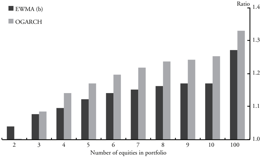
Chart 19 VaR Violation Ratios for Portfolio of Equities(a)
